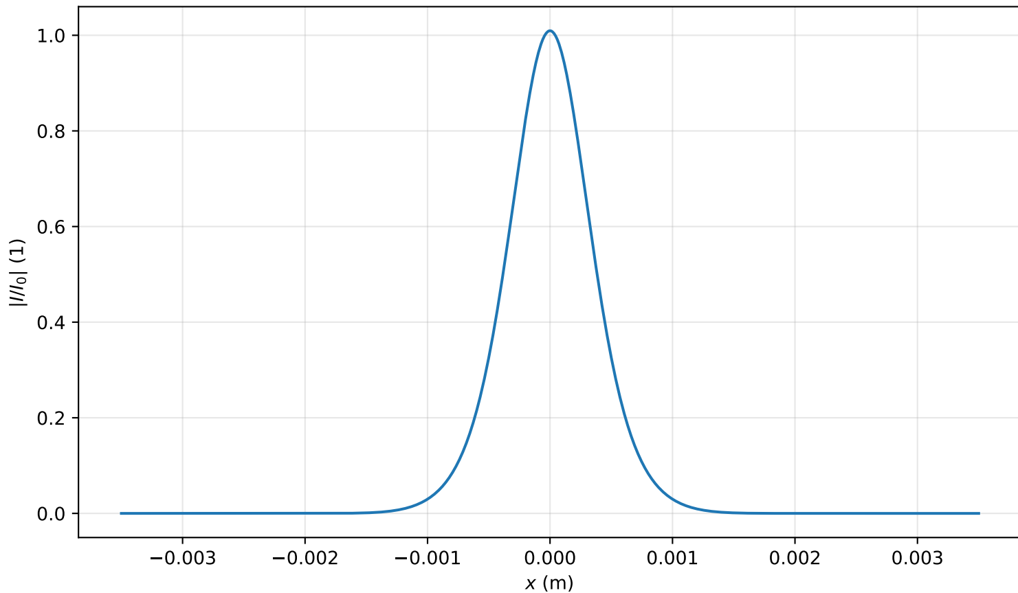
Intensity profile I(x, y = 0, z = 1.274m)/I_0 , P_{in}=0.5P_{cr} , artificial time
